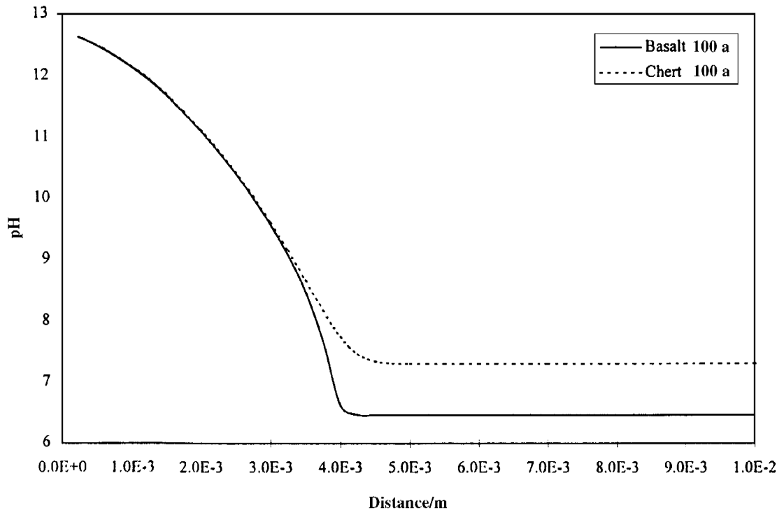
Figure 7-21. A comparison of pH profiles for basalt and chert at 100 years (MARQUISS).
