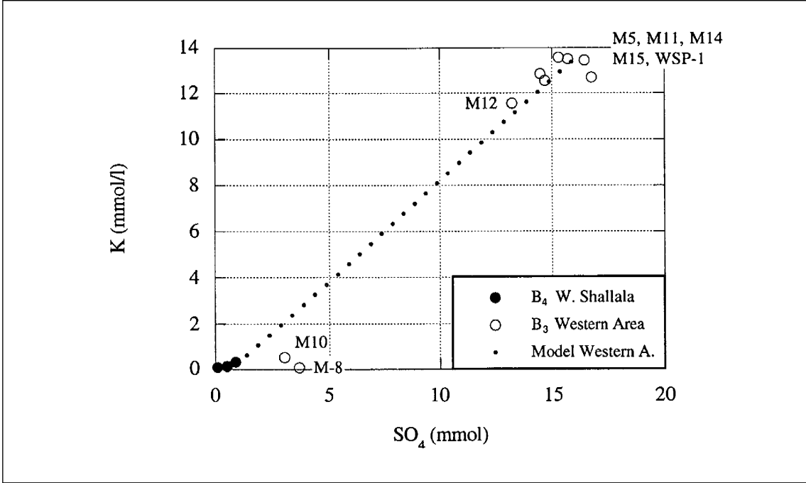
Figure 6-17. Calculated evolution of \text{K}^+ and \text{SO}_4^{2-} concentrations compared with measured data of high-pH groundwaters from the Western Springs area.
